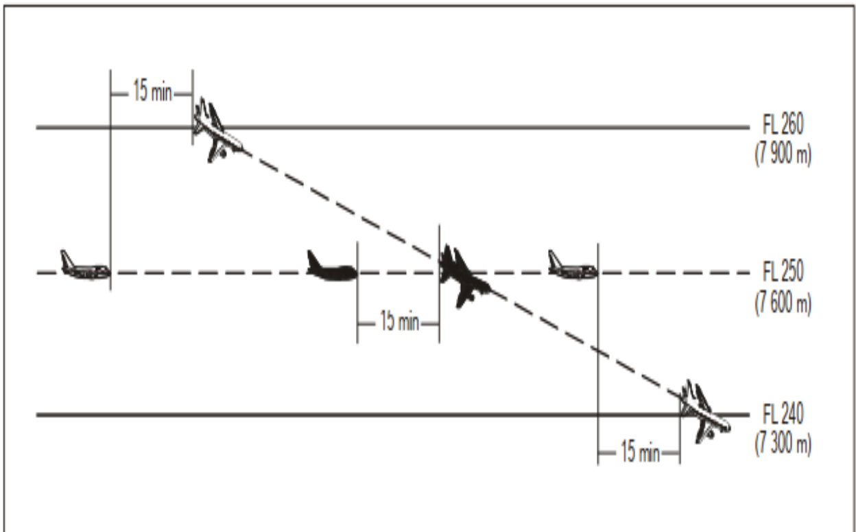
Figure 5-19B. Fifteen-minute separation between aircraft descending and on crossing tracks (see 5.4.2.2.2.2 a))
