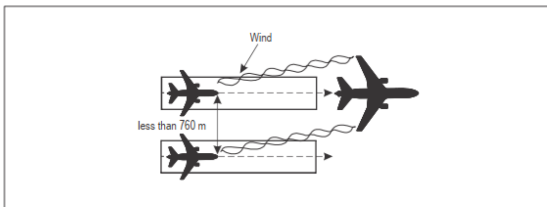
Figure 5-42. Wake turbulence separation for following aircraft (see 5.8.3.1 a) and b) and 5.8.3.2 a) and b))
