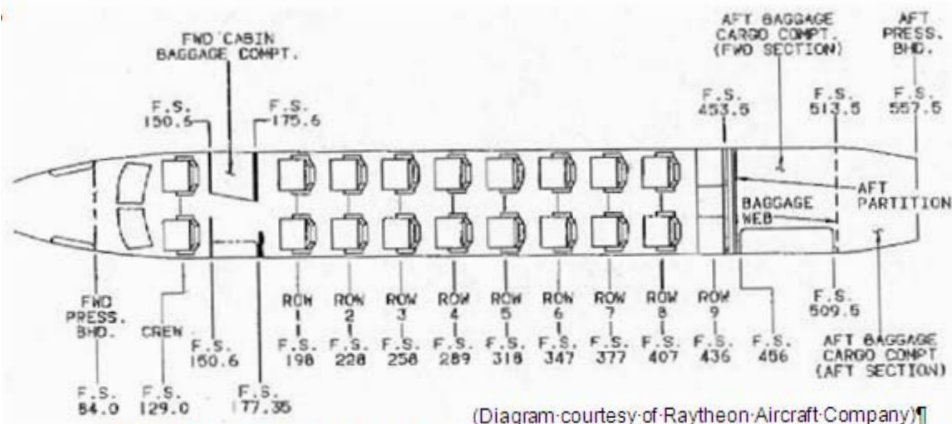
FIGURE 3-1. SAMPLE AIRCRAFT INTERIOR SEATING DIAGRAM
